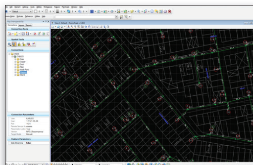
Existing telecommunications infrastructure was mapped out using Bentley Map, and then a modified network was designed with Fiber Deep architecture in Bentley Coax and Bentley Fiber.
