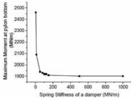
Fig. 6: Maximum moment at pylon bottom
