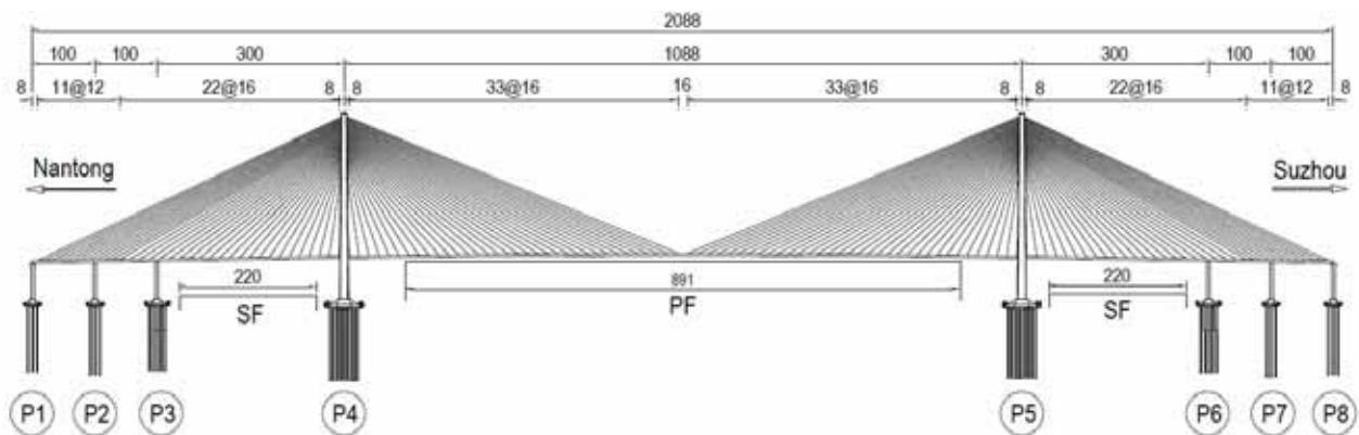
Fig. 1: Span Arrangement (unit: m)
