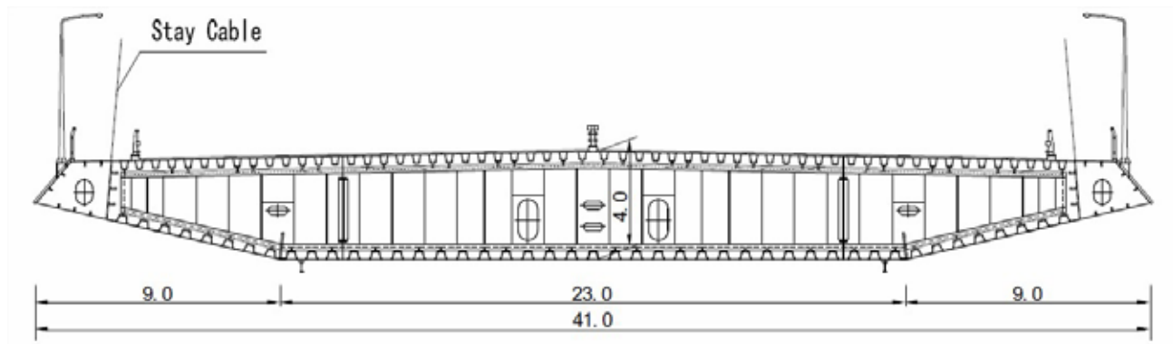
Fig. 2: Cross Section of the Girder (unit: m)
