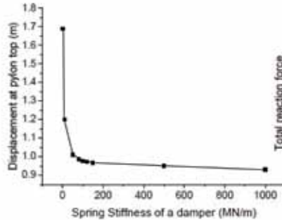
Fig. 7: Displacement at pylon top
