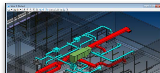
HVAC components are integrated with piping for robust plant design.
