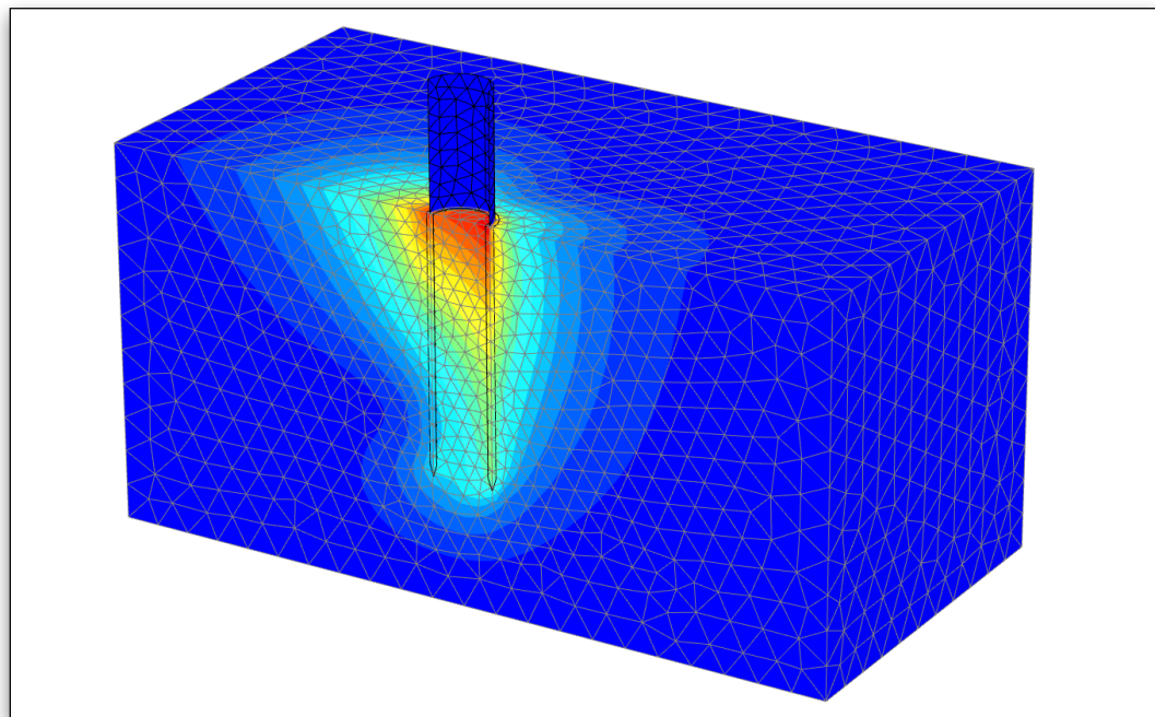
Field of displacements for a laterally loaded monopile.
