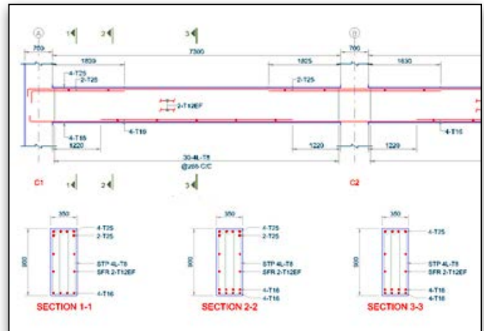
Concrete design and documentation in RCDC® working directly off the RAM model.
