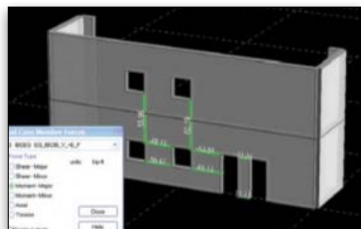
Shear wall forces displayed at any cross section.
