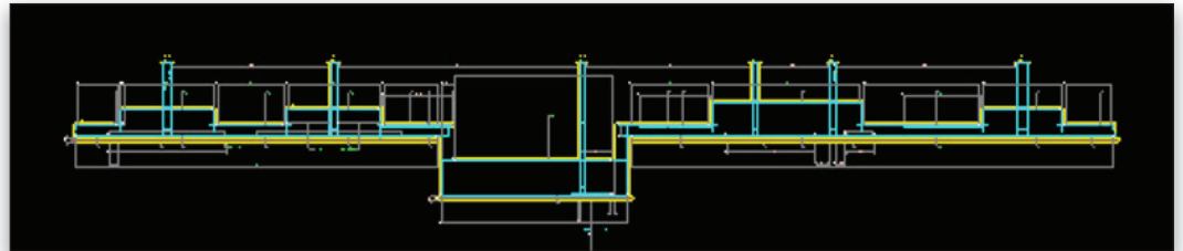
Cross section through a raft/mat foundation
