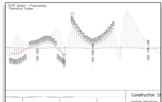
Camber line.
