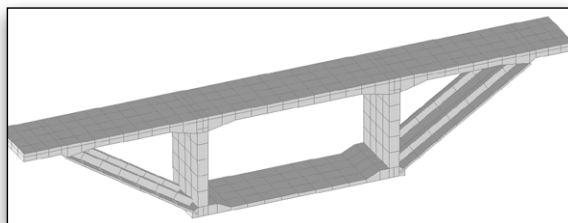
Composite cross-section.
