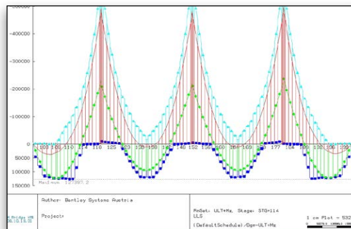
Steel stresses due to ULS in composite girder.
