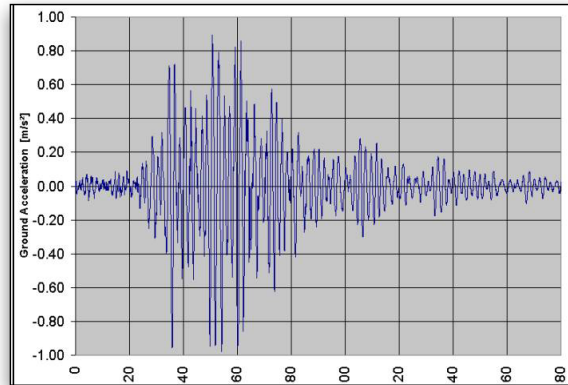
Acceleration diagram – time history calculation.
